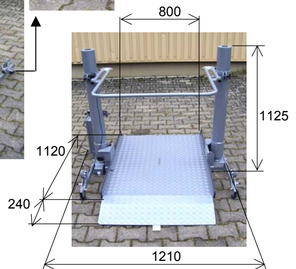
Klapprollen-Set (Option)
